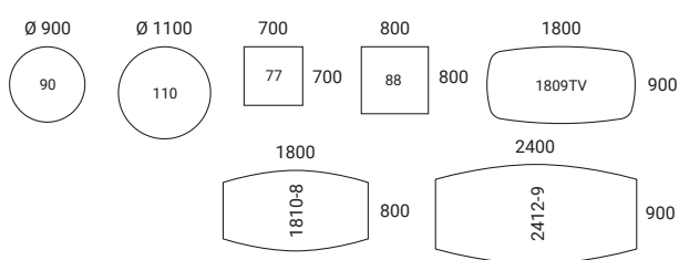
MEETING TABLE Height 900 mm
